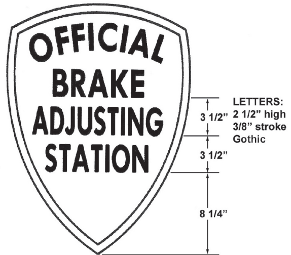
FIGURE 2. LETTERING DIMENSIONS
